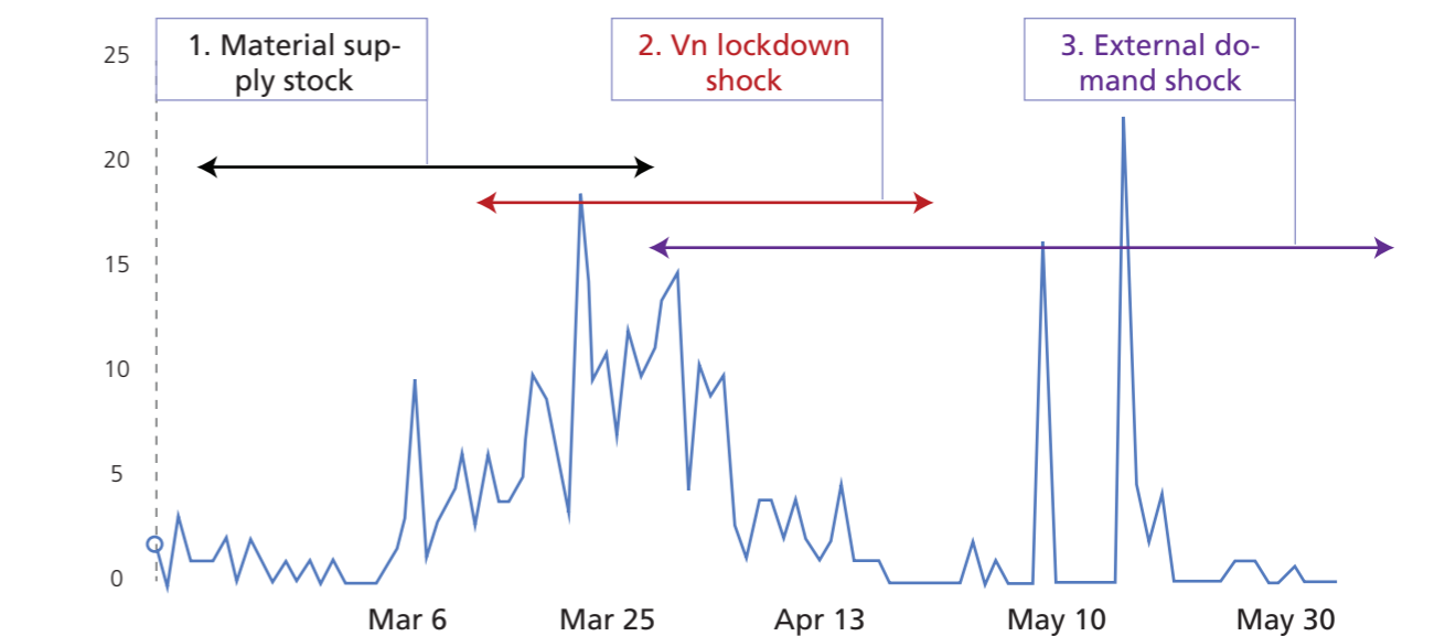
Figure 3: Three economic shocks to the manufacturing sector of Vietnam
